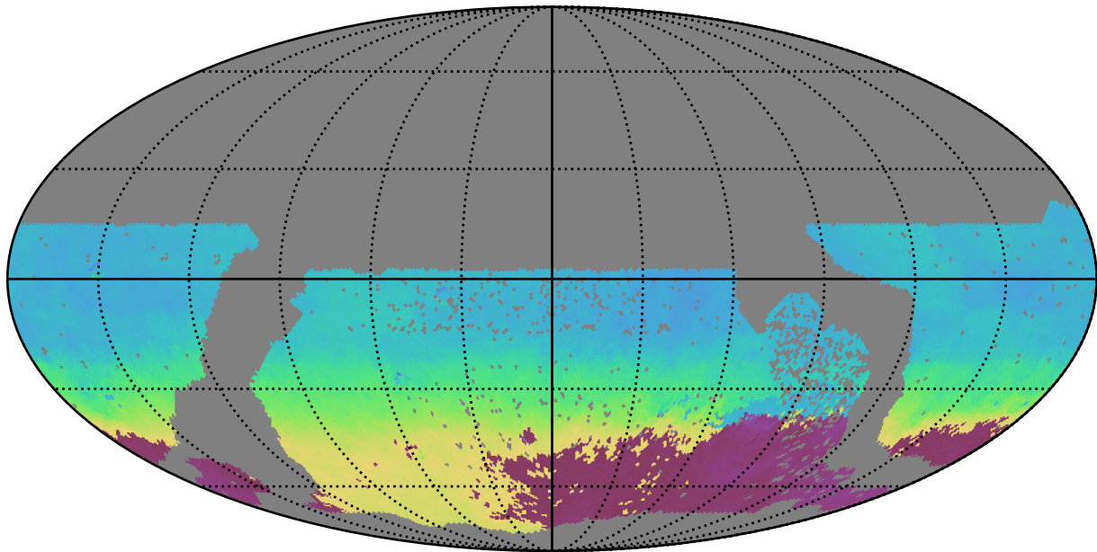
no_high_blob_v3.3_10yrs WFD r band: AngleMean rotSkyPos
