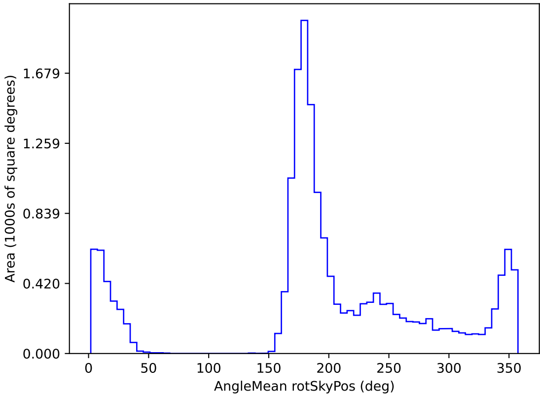
no_high_blob_v3.3_10yrs WFD r band: AngleMean rotSkyPos
