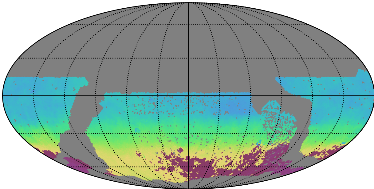
no_high_blob_v3.3_10yrs WFD i band: AngleMean rotSkyPos
