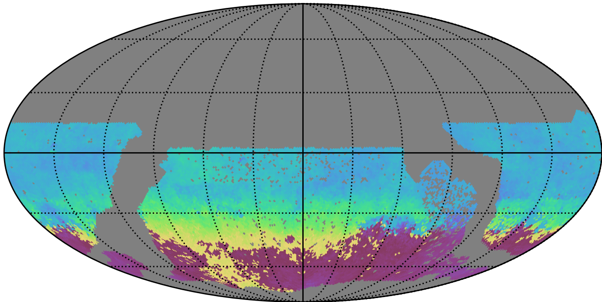
no_high_blob_v3.3_10yrs WFD g band: AngleMean rotSkyPos
