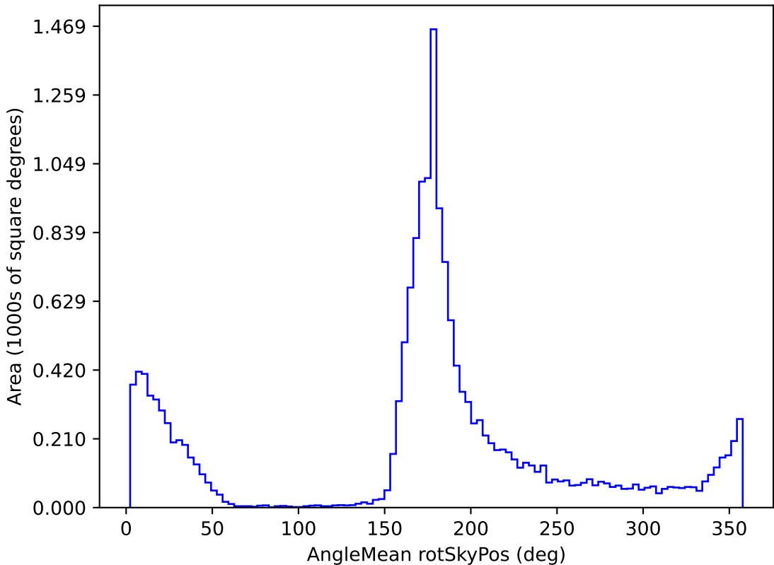
no_high_blob_v3.3_10yrs WFD g band: AngleMean rotSkyPos
