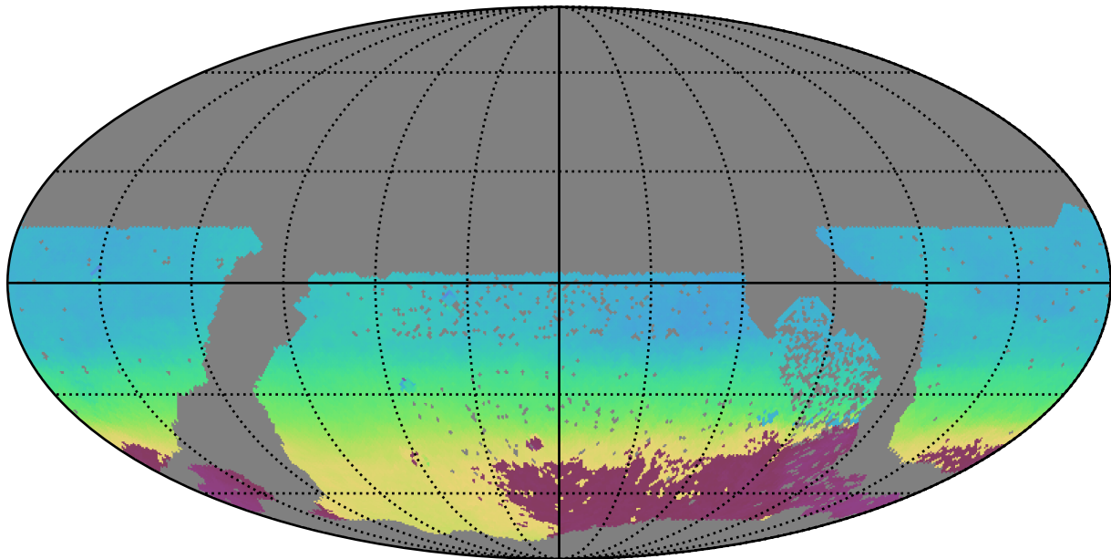
no_high_blob_v3.3_10yrs WFD all bands: AngleMean rotSkyPos
