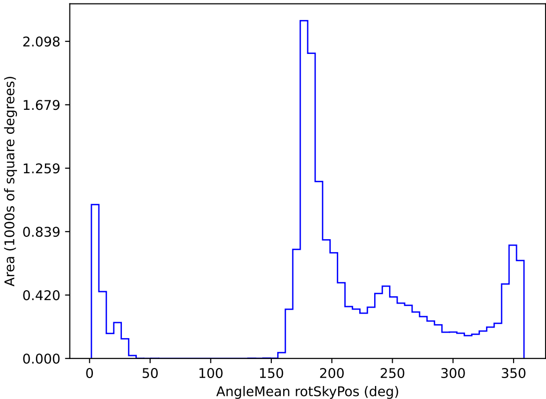
no_high_blob_v3.3_10yrs WFD all bands: AngleMean rotSkyPos
