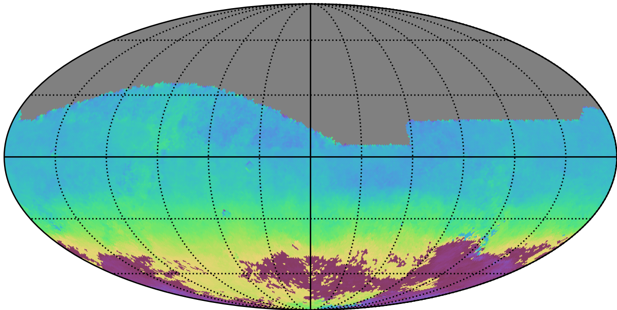
no_high_blob_v3.3_10yrs All sky z band: AngleMean rotSkyPos
