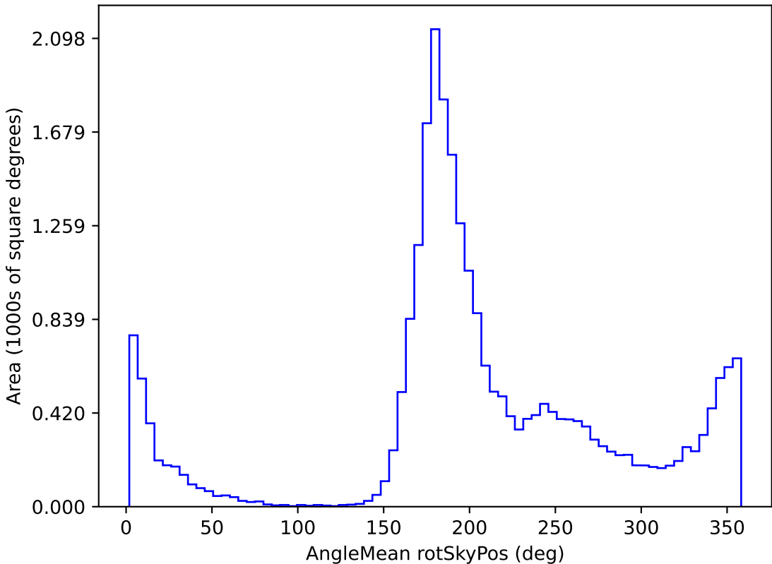
no_high_blob_v3.3_10yrs All sky z band: AngleMean rotSkyPos
