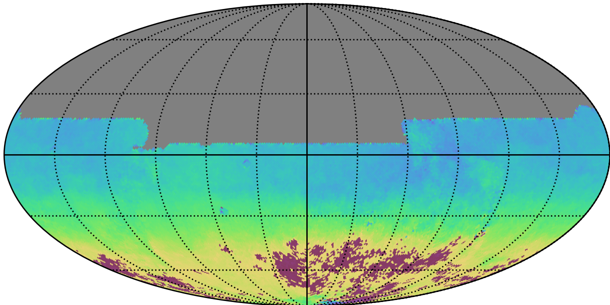
no_high_blob_v3.3_10yrs All sky y band: AngleMean rotSkyPos
