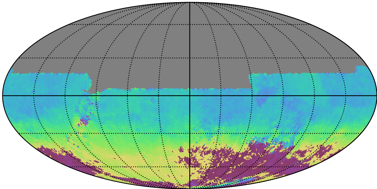
no_high_blob_v3.3_10yrs All sky u band: AngleMean rotSkyPos
