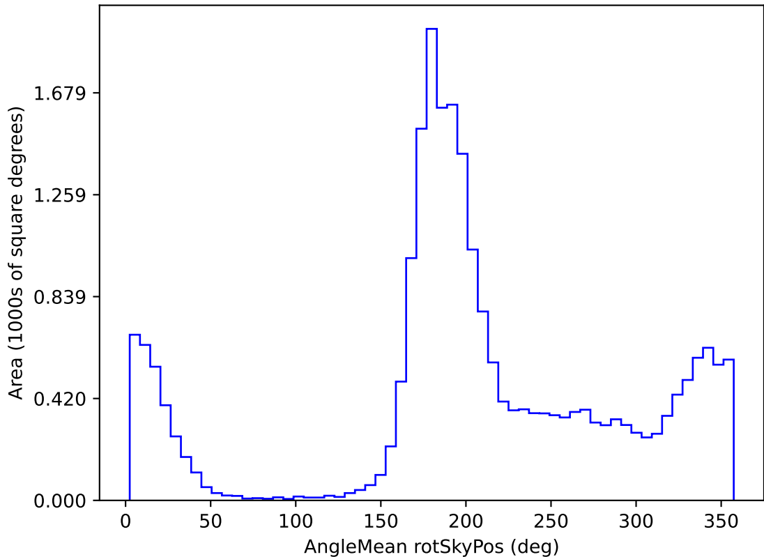
no_high_blob_v3.3_10yrs All sky u band: AngleMean rotSkyPos
