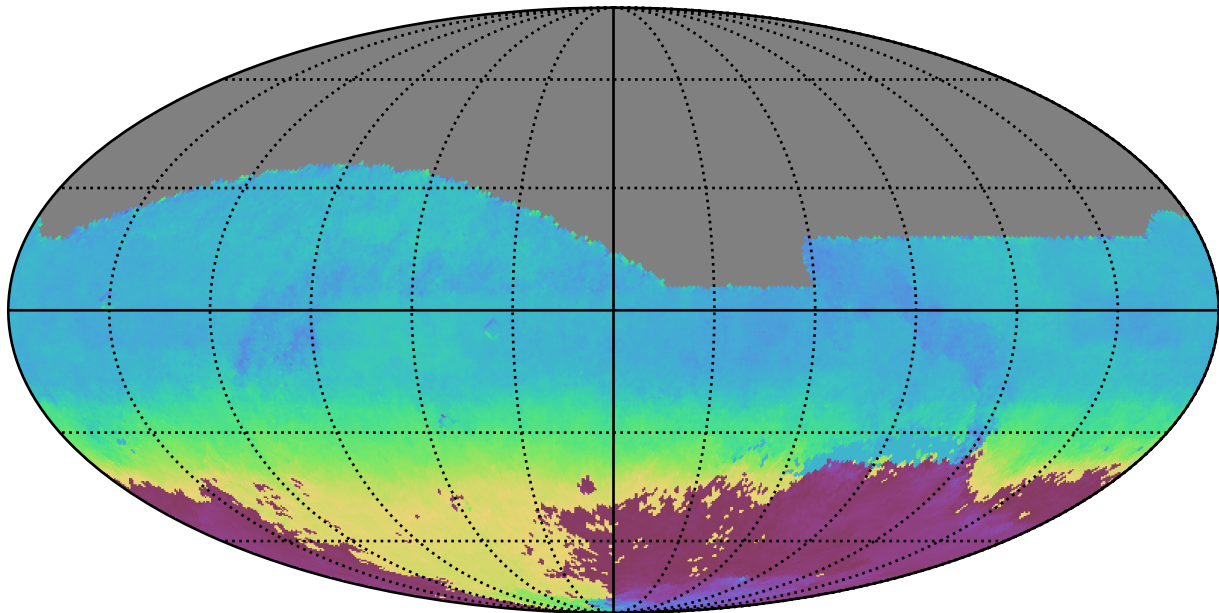
no_high_blob_v3.3_10yrs All sky r band: AngleMean rotSkyPos
