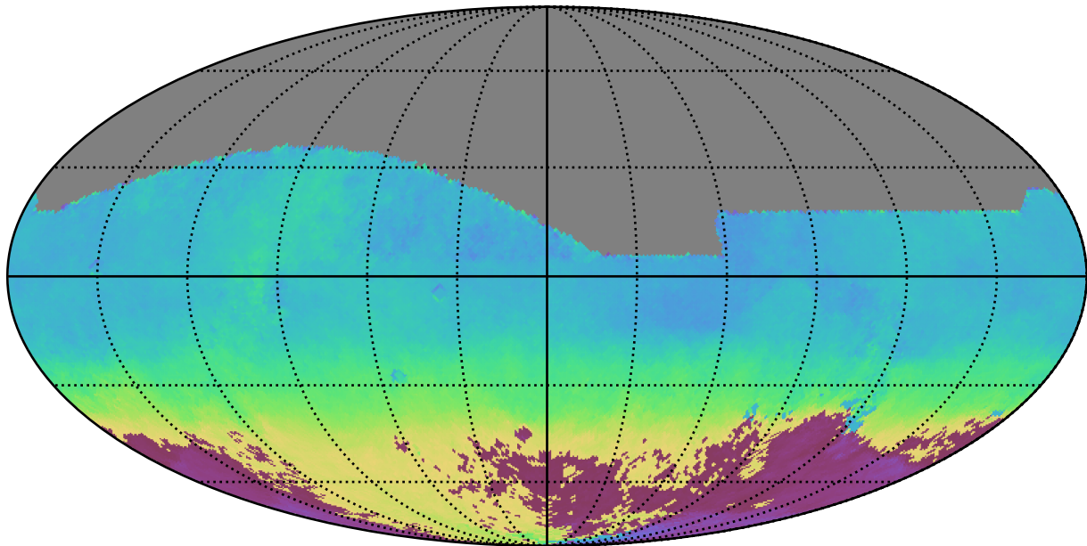
no_high_blob_v3.3_10yrs All sky i band: AngleMean rotSkyPos
