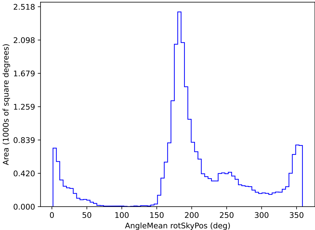
no_high_blob_v3.3_10yrs All sky i band: AngleMean rotSkyPos
