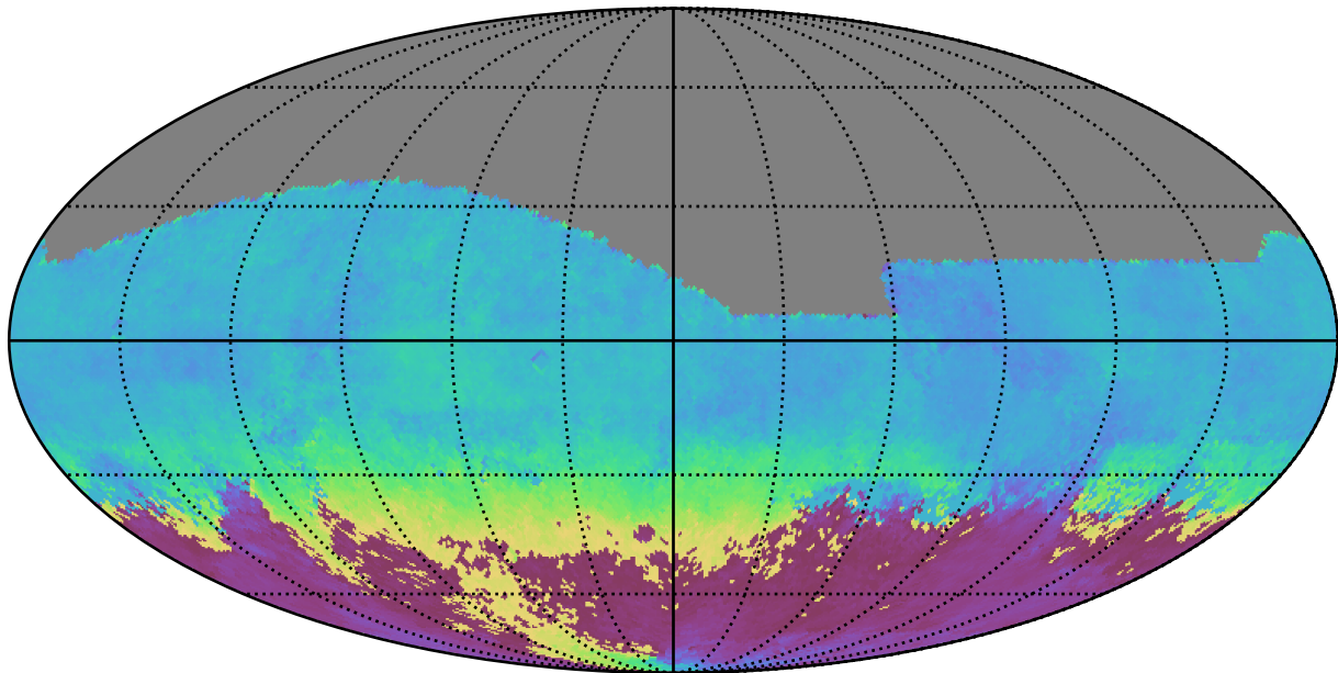
no_high_blob_v3.3_10yrs All sky g band: AngleMean rotSkyPos
