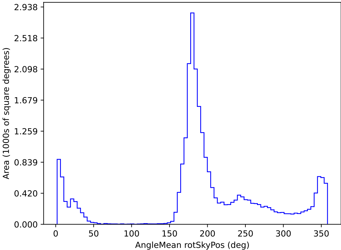
no_high_blob_v3.3_10yrs All sky all bands: AngleMean rotSkyPos
