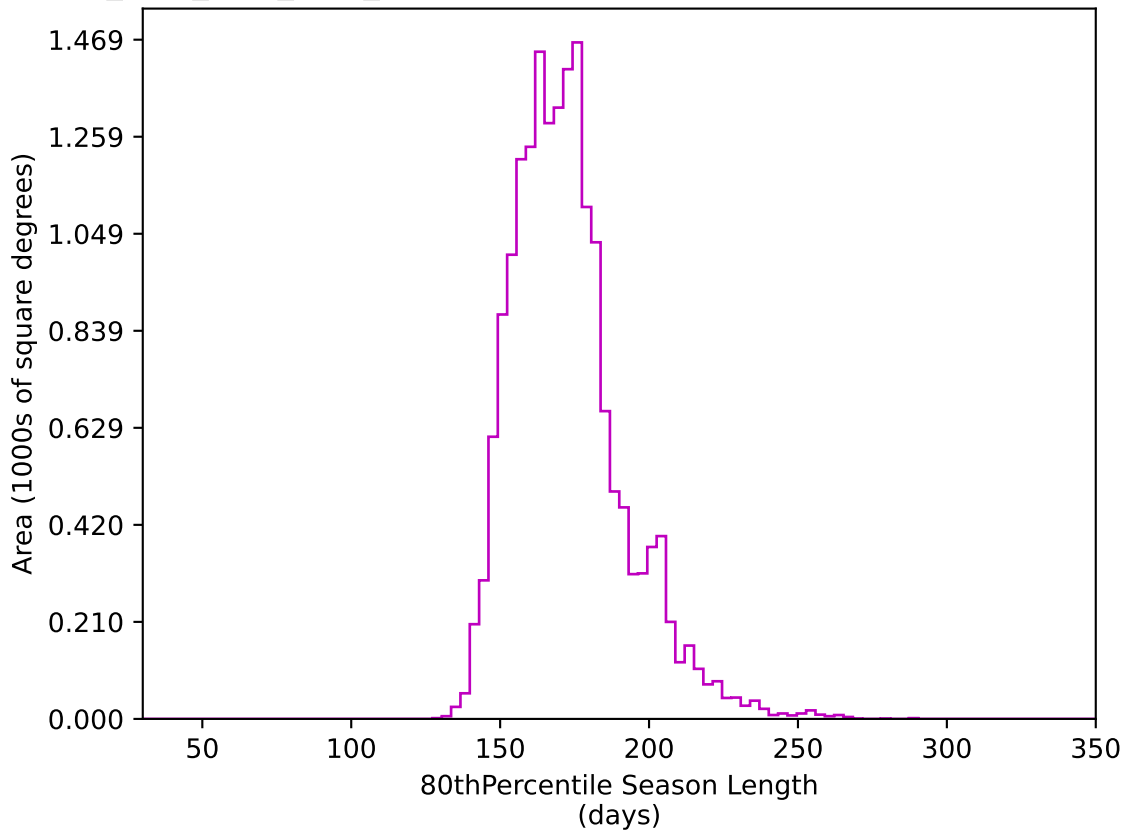
no_high_blob_v3.3_10yrs WFD z band: 80thPercentile Season Length
