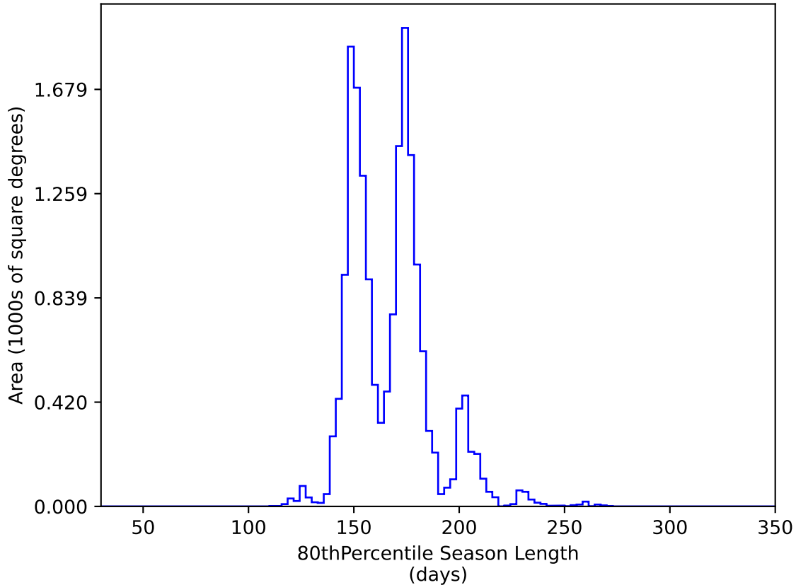
no_high_blob_v3.3_10yrs WFD y band: 80thPercentile Season Length
