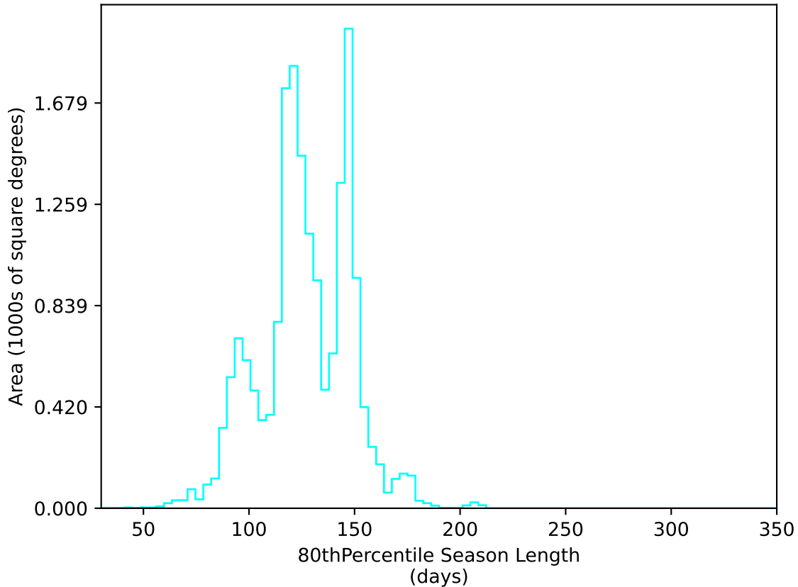
no_high_blob_v3.3_10yrs WFD u band: 80thPercentile Season Length
