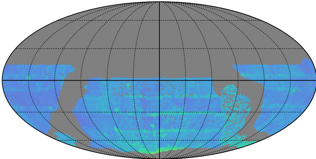
no_high_blob_v3.3_10yrs WFD r band: 80thPercentile Season Length
