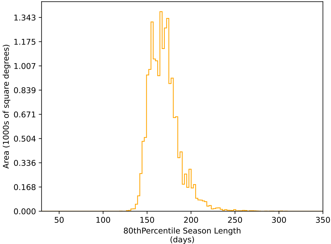
no_high_blob_v3.3_10yrs WFD r band: 80thPercentile Season Length
