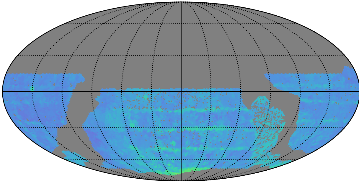
no_high_blob_v3.3_10yrs WFD i band: 80thPercentile Season Length
