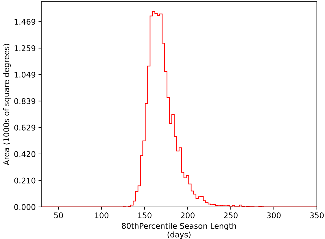
no_high_blob_v3.3_10yrs WFD i band: 80thPercentile Season Length
