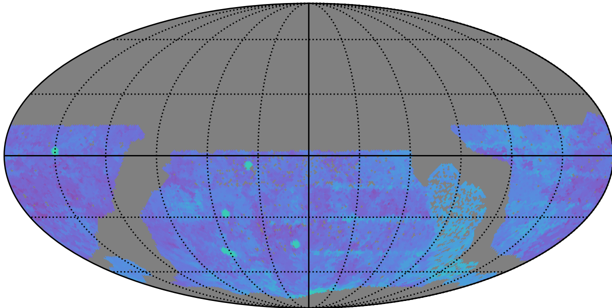
no_high_blob_v3.3_10yrs WFD g band: 80thPercentile Season Length
