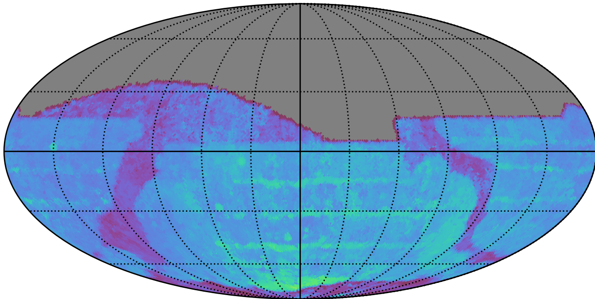
no_high_blob_v3.3_10yrs All sky z band: 80thPercentile Season Length
