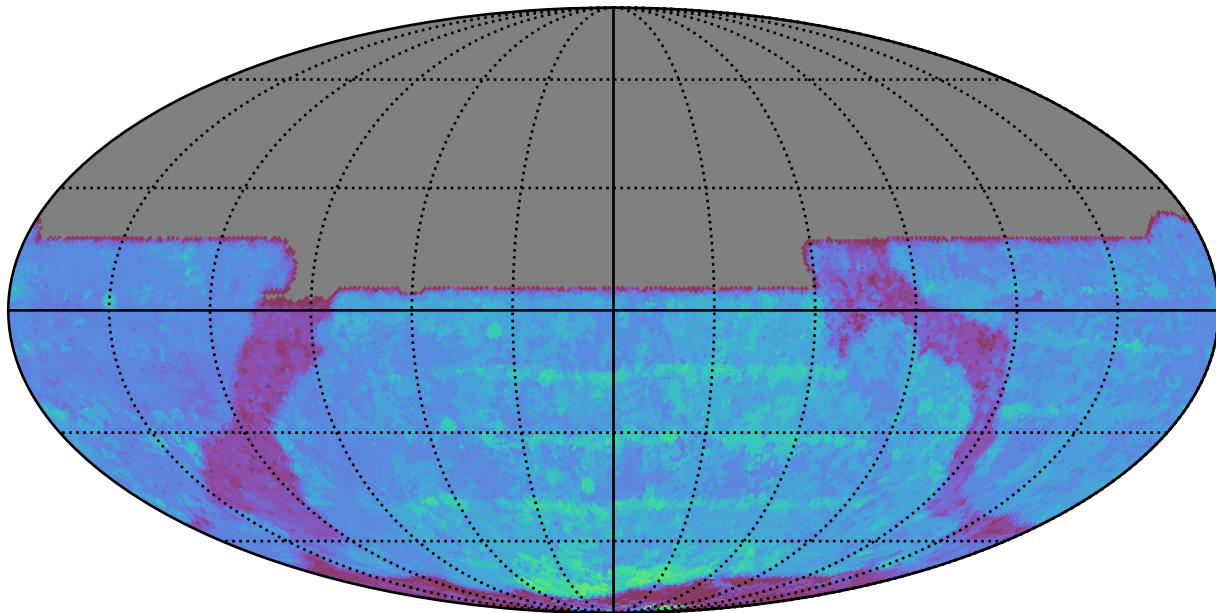
no_high_blob_v3.3_10yrs All sky y band: 80thPercentile Season Length
