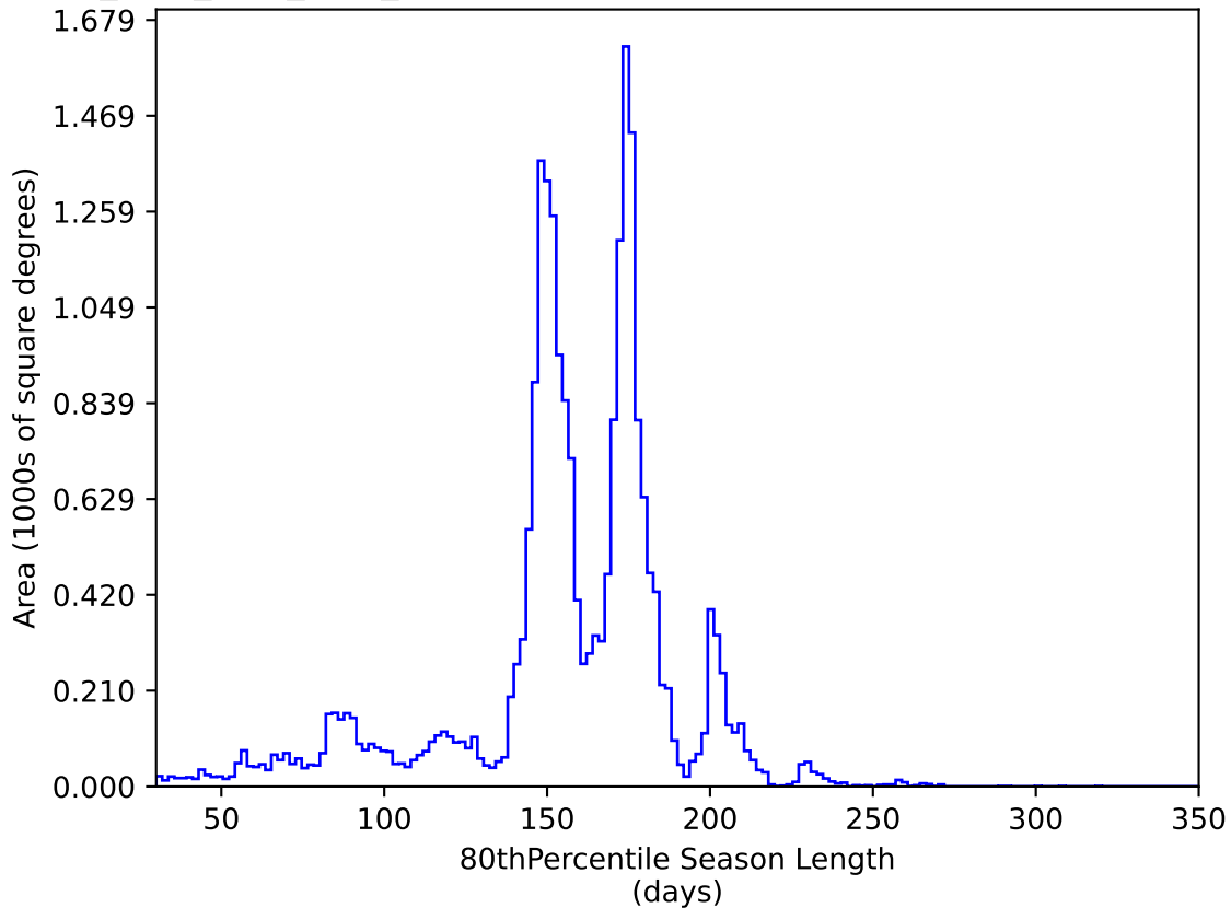
no_high_blob_v3.3_10yrs All sky y band: 80thPercentile Season Length
