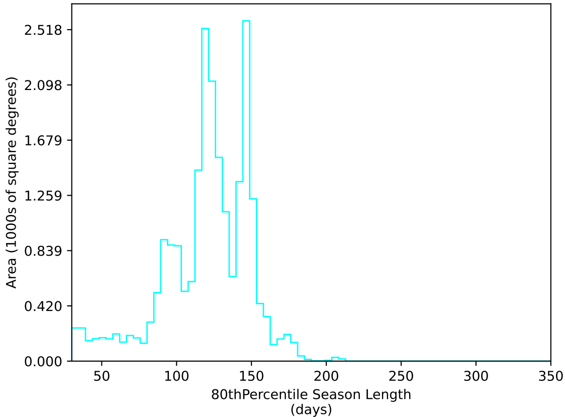
no_high_blob_v3.3_10yrs All sky u band: 80thPercentile Season Length
