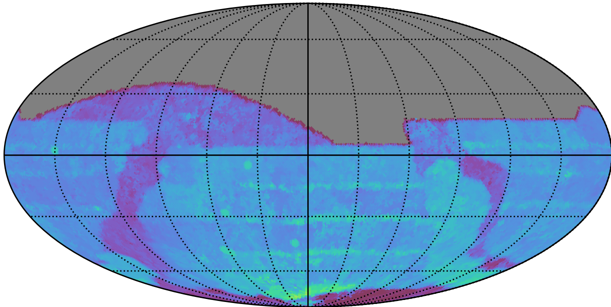
no_high_blob_v3.3_10yrs All sky r band: 80thPercentile Season Length
