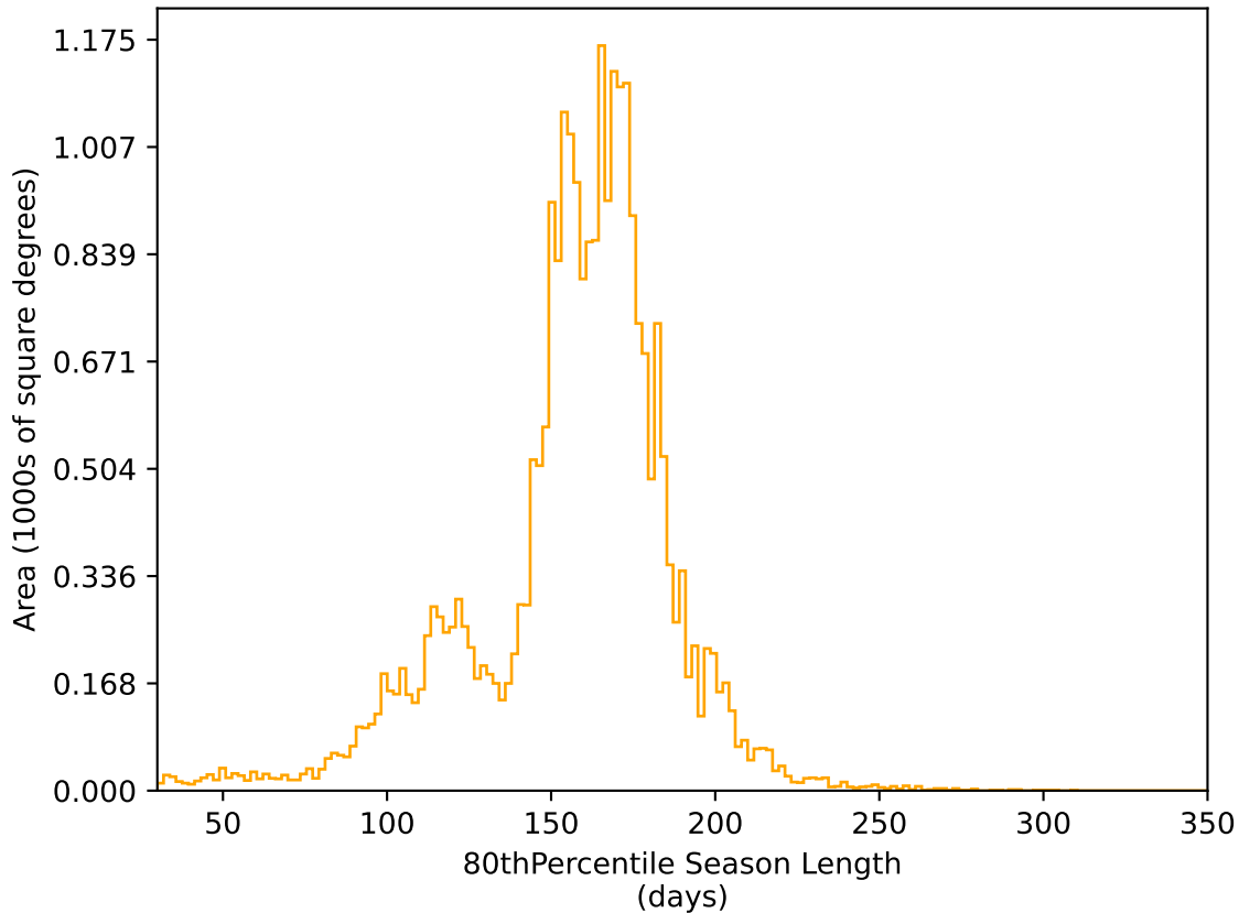
no_high_blob_v3.3_10yrs All sky r band: 80thPercentile Season Length
