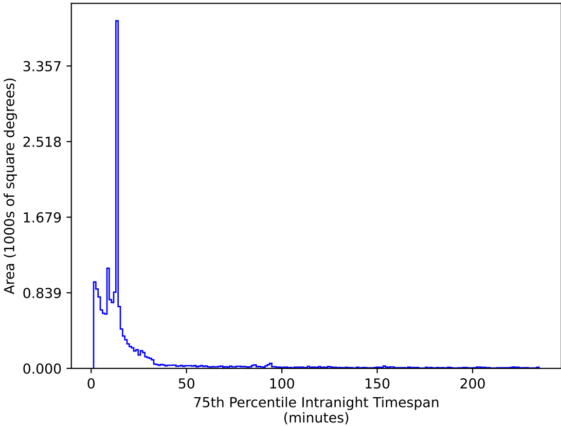
no_high_blob_v3.3_10yrs WFD z band: 75th Percentile Intranight Timespan
