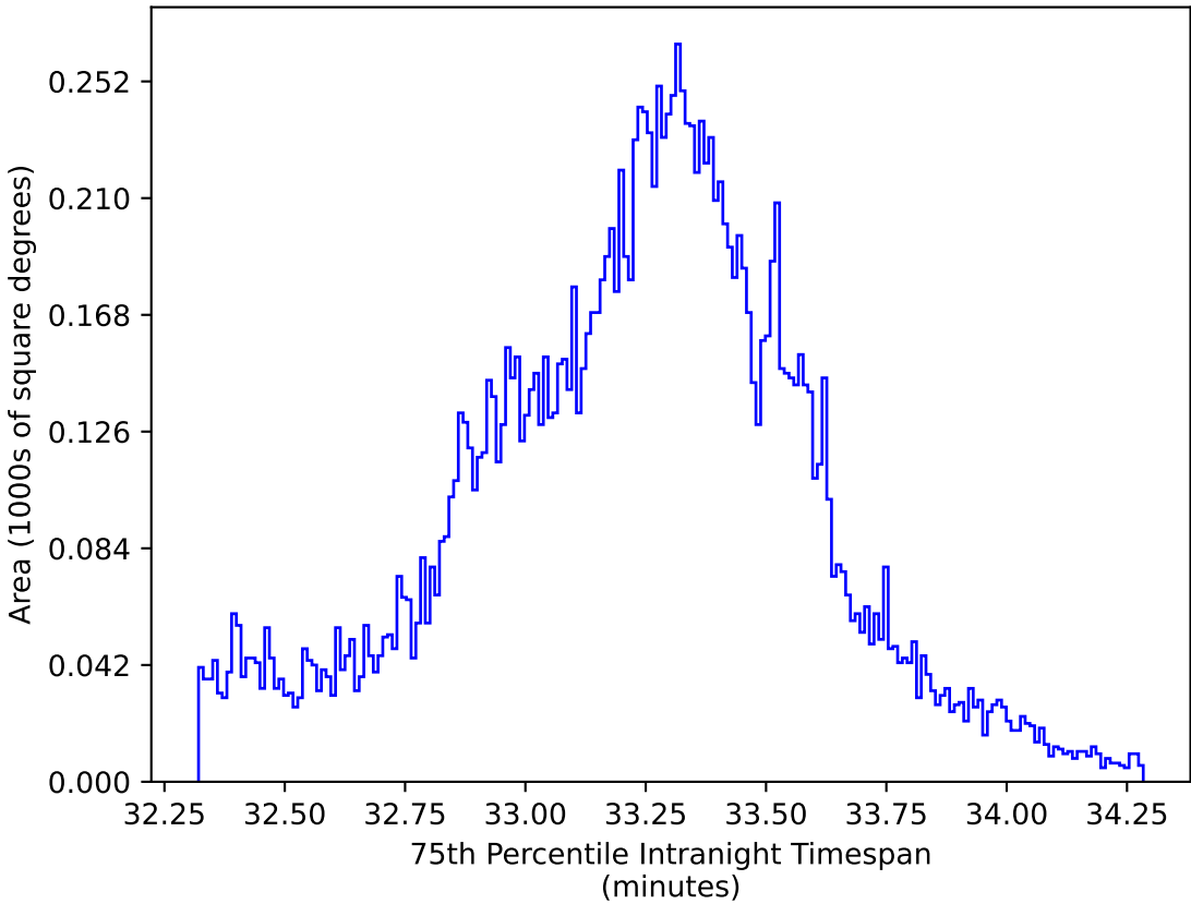
no_high_blob_v3.3_10yrs WFD y band: 75th Percentile Intranight Timespan
