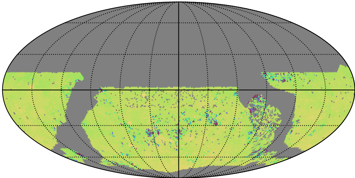
no_high_blob_v3.3_10yrs WFD ug bands: 75th Percentile Intranight Timespan
