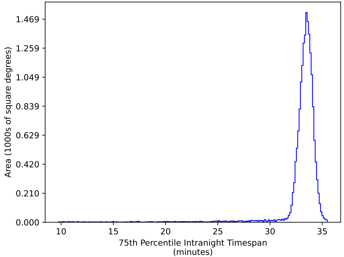
no_high_blob_v3.3_10yrs WFD ug bands: 75th Percentile Intranight Timespan
