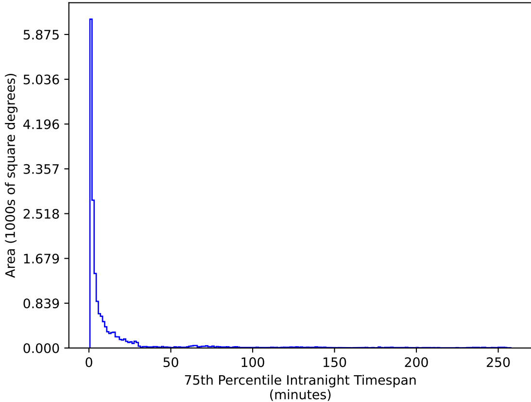
no_high_blob_v3.3_10yrs WFD u band: 75th Percentile Intranight Timespan
