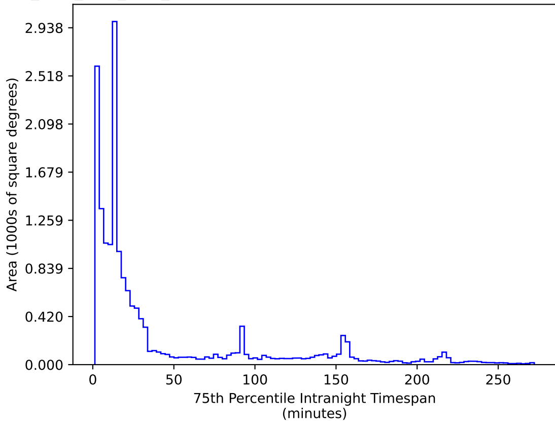
no_high_blob_v3.3_10yrs WFD r band: 75th Percentile Intranight Timespan
