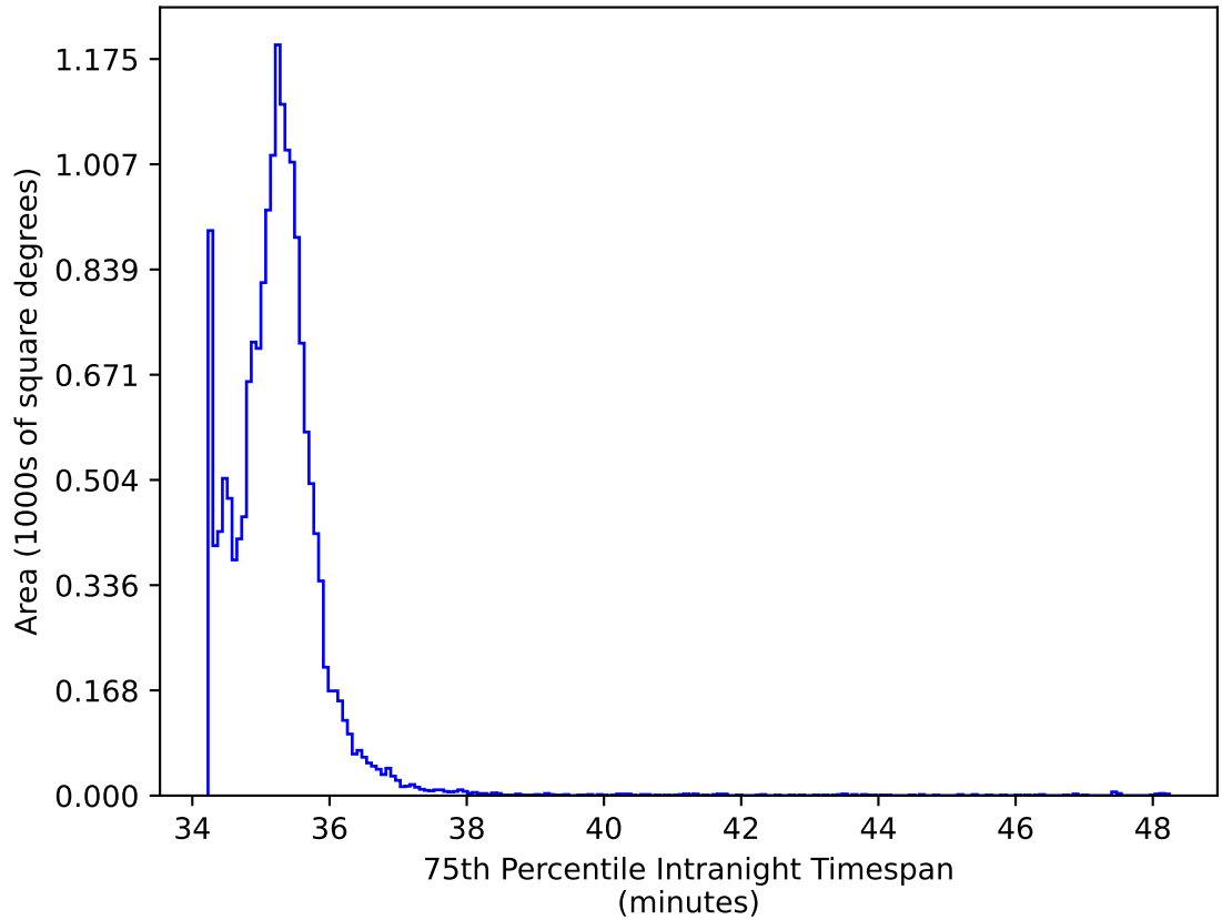
no_high_blob_v3.3_10yrs WFD iz bands: 75th Percentile Intranight Timespan
