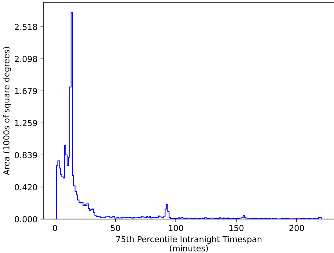
no_high_blob_v3.3_10yrs WFD i band: 75th Percentile Intranight Timespan
