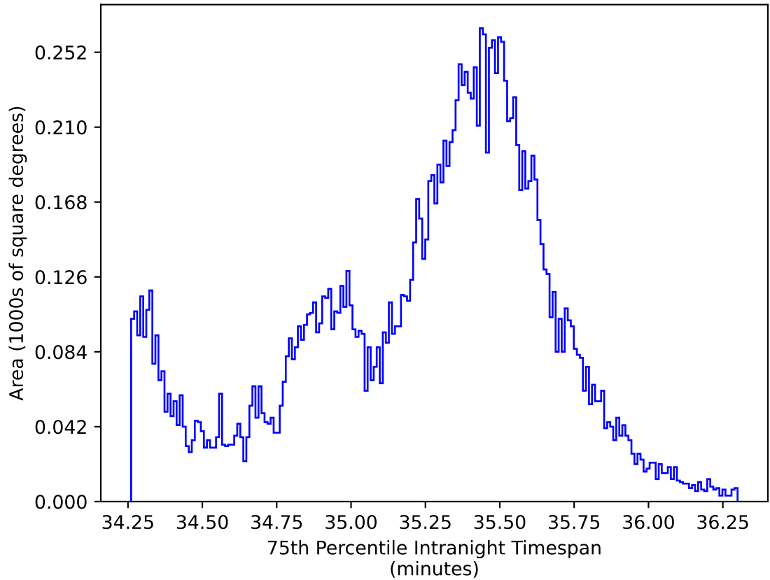
no_high_blob_v3.3_10yrs WFD all bands: 75th Percentile Intranight Timespan
