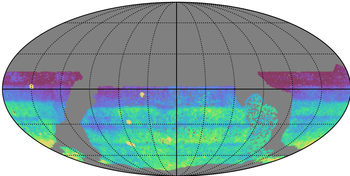
no_high_blob_v3.3_10yrs WFD: 75th Percentile Intranight Timespan
