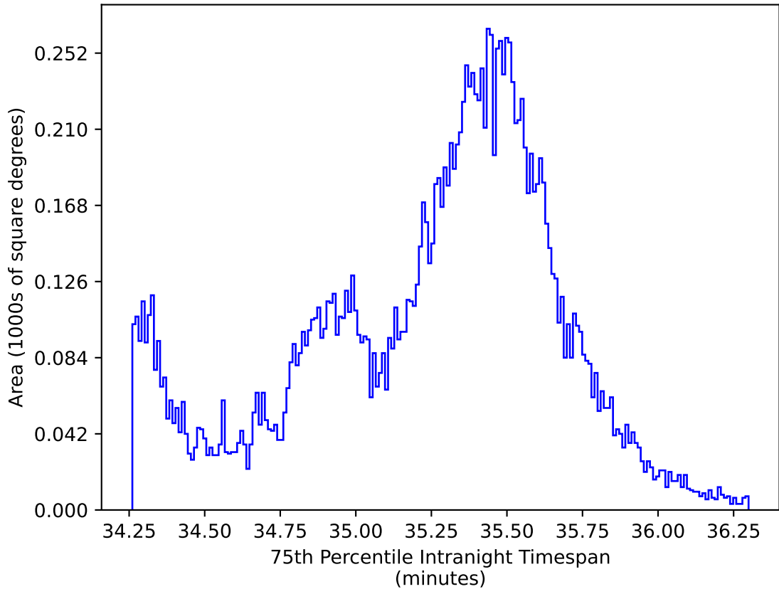
no_high_blob_v3.3_10yrs WFD: 75th Percentile Intranight Timespan
