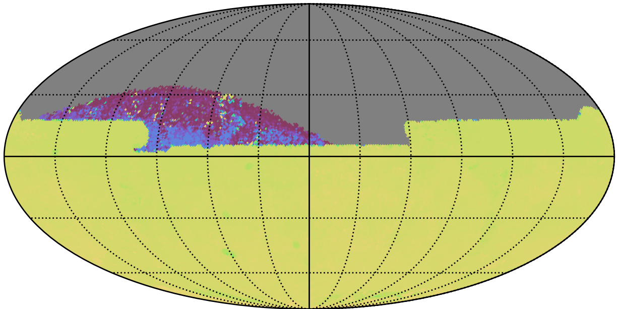
no_high_blob_v3.3_10yrs All sky zy bands: 75th Percentile Intranight Timespan
