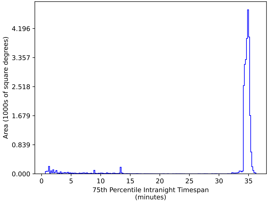
no_high_blob_v3.3_10yrs All sky zy bands: 75th Percentile Intranight Timespan
