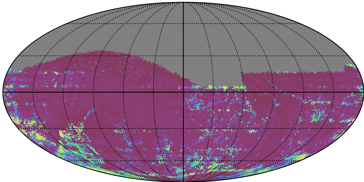
no_high_blob_v3.3_10yrs All sky z band: 75th Percentile Intranight Timespan
