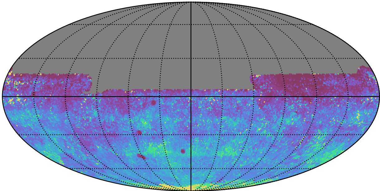
no_high_blob_v3.3_10yrs All sky y band: 75th Percentile Intranight Timespan
