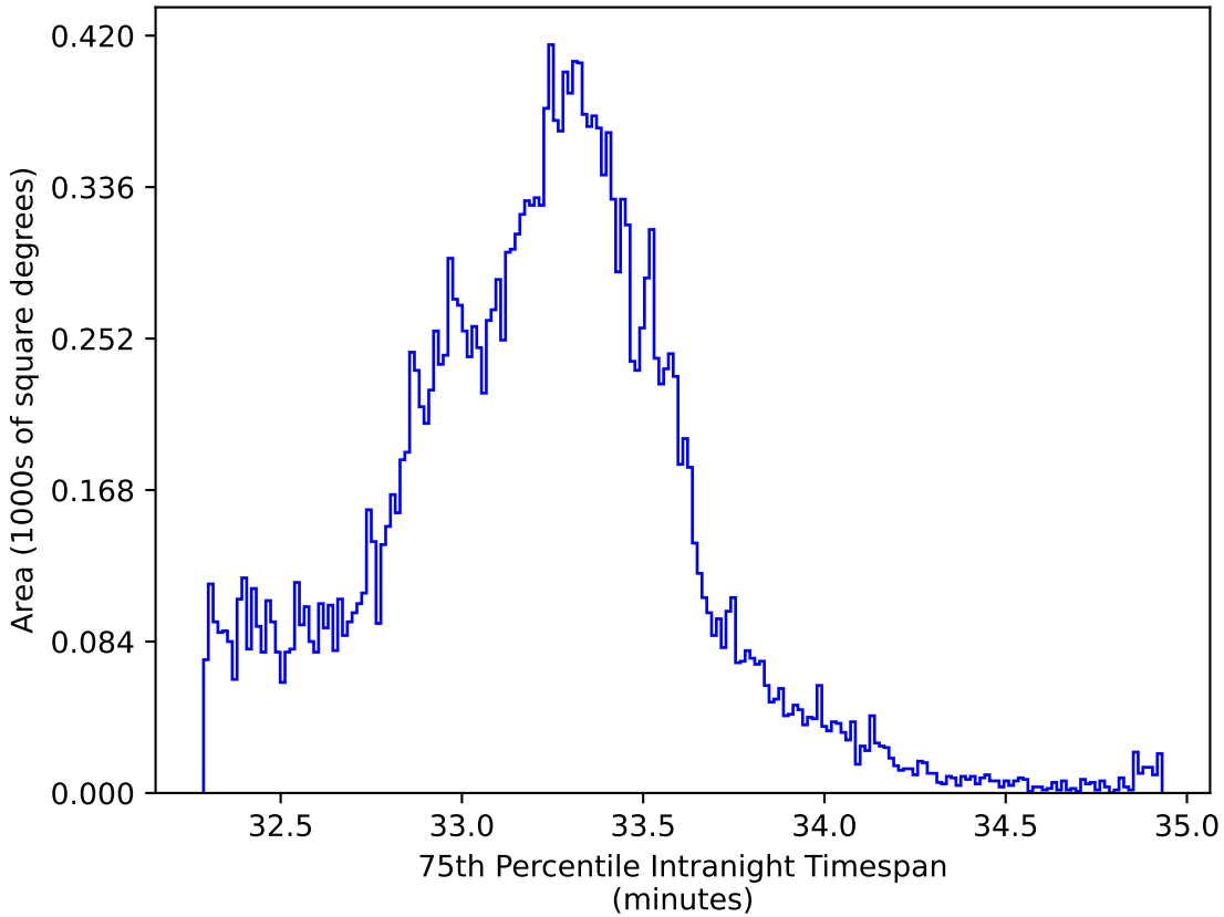
no_high_blob_v3.3_10yrs All sky y band: 75th Percentile Intranight Timespan
