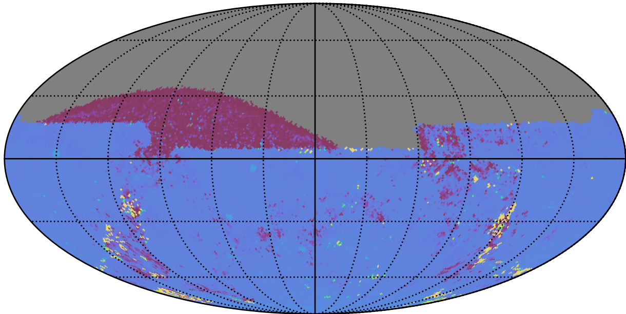
no_high_blob_v3.3_10yrs All sky ug bands: 75th Percentile Intranight Timespan
