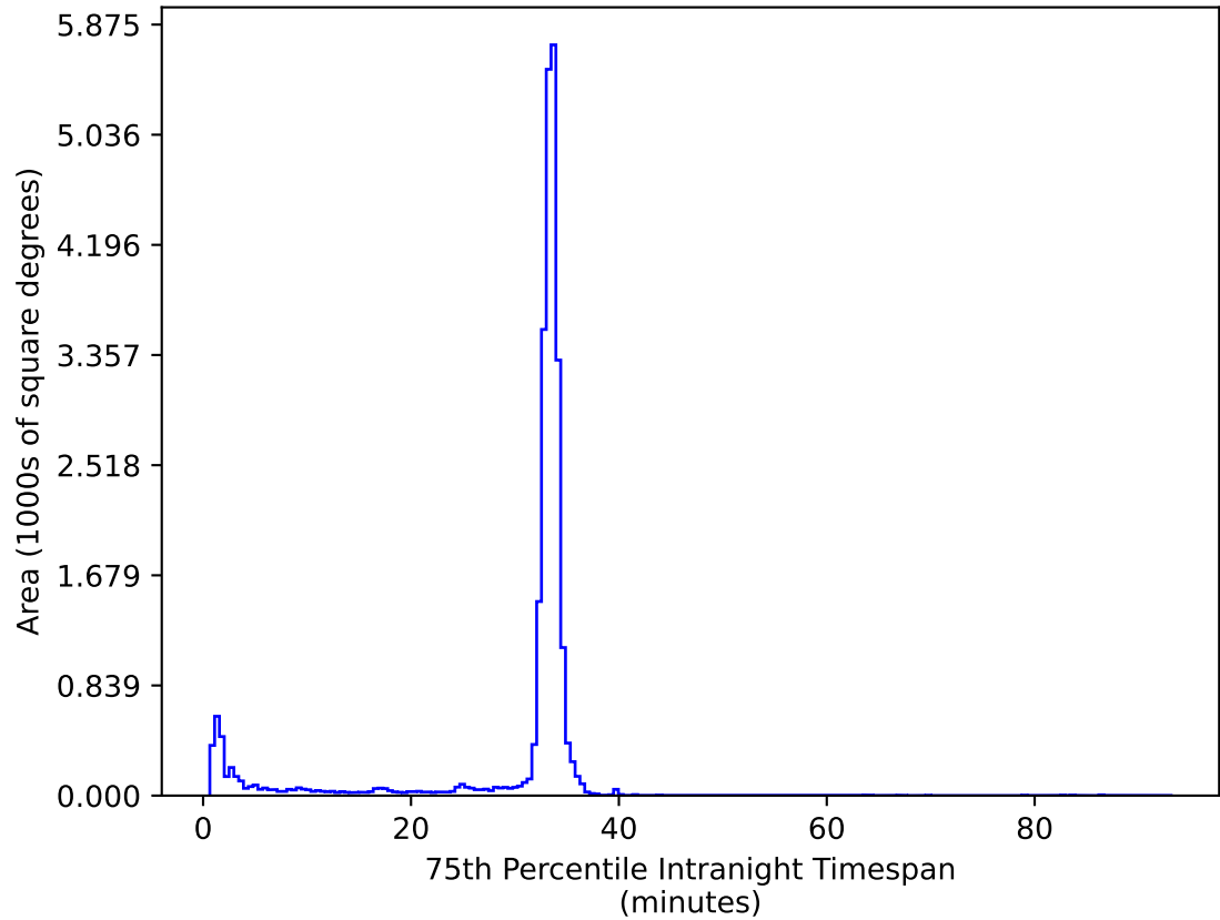
no_high_blob_v3.3_10yrs All sky ug bands: 75th Percentile Intranight Timespan
