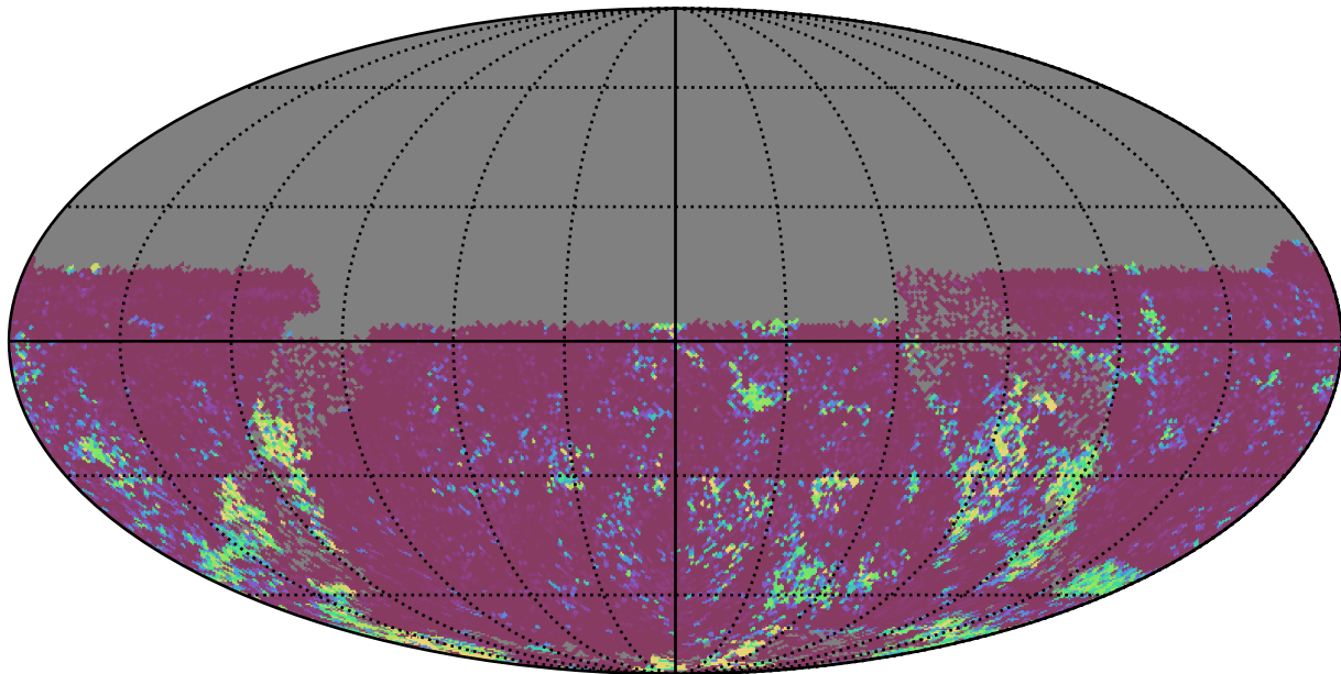
no_high_blob_v3.3_10yrs All sky u band: 75th Percentile Intranight Timespan
